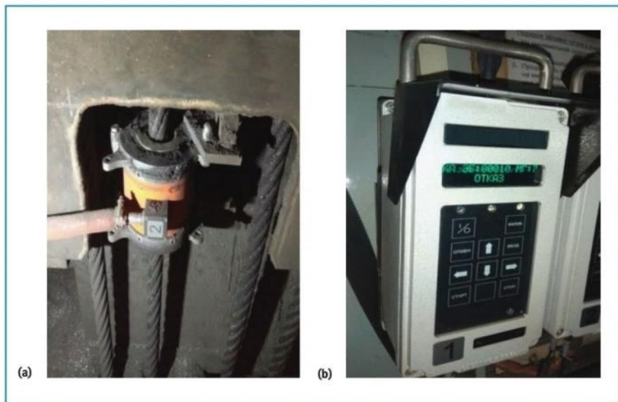
Figure 7. Components of the automated condition monitoring system: (a) magnetic head permanently installed on the rope; (b) control and display unit in the cabin of the crane's operator.
