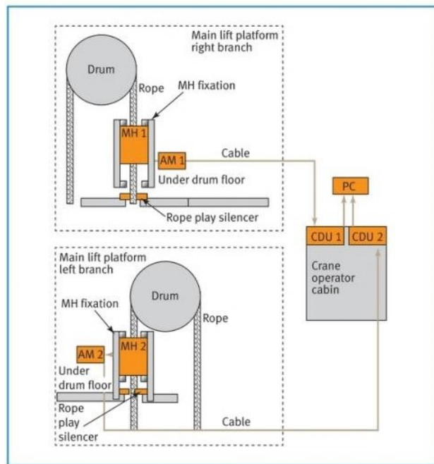
Figure 6. Installation schematic of the automated condition monitoring system for ladle crane ropes (MH = magnetic head; AM = analog module).
