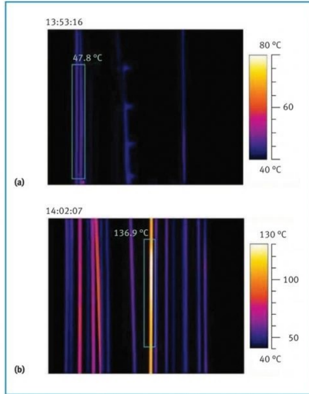
Figure 3. Thermograms of ladle crane ropes: (a) before pouring; (b) after pouring.
