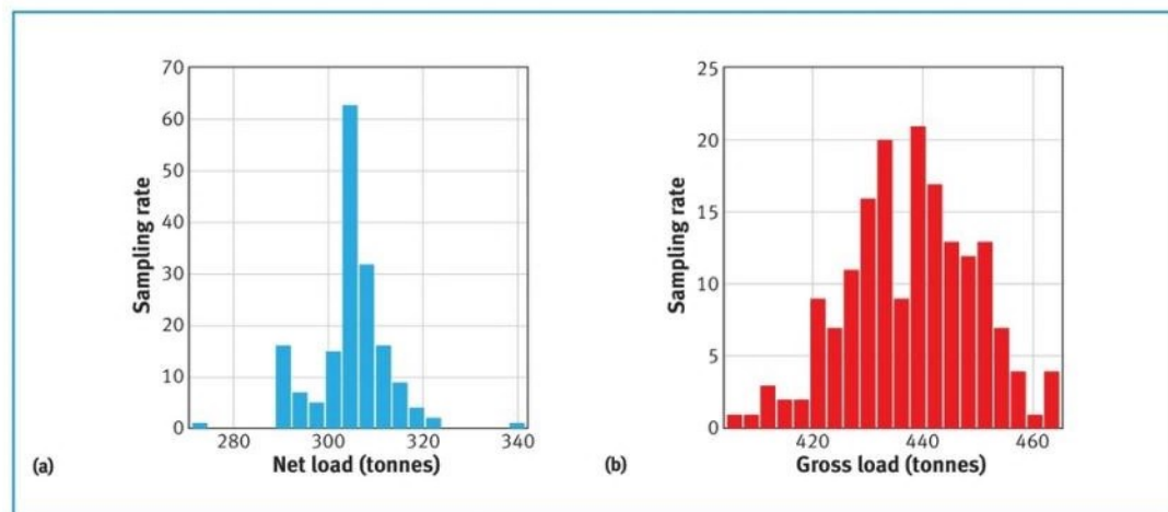
Figure 2. Histograms displaying the loads on ladle ropes: (a) net load; (b) gross load.
