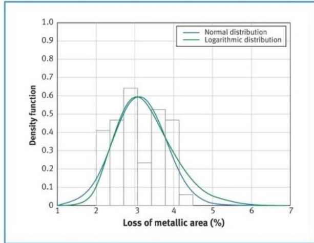
Figure 10. Histogram of the LMA value at rope discard and its approximations.
