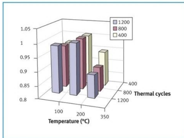
Figure 4. Relative change in wire tensile strength during different thermal cycles.
