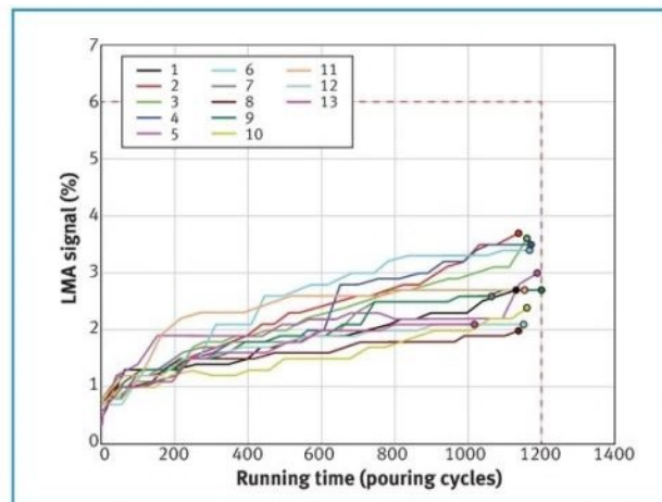
Figure 9. LMA based on running time of EN 12385-4-2000 ropes on crane 10, from 18 October 2017 to 20 October 2019.
