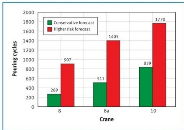
Figure 11. Potential extended lifetime of the ropes, provided that the LMA growth is extrapolated from the last three inspections.
