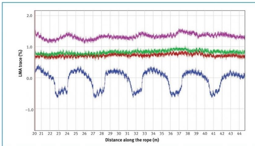
Figure 8. LMA traces from the working section of a rope installed on crane 10 recorded from 1–12 March 2020.
